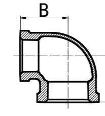
Reducing Elbow, 90°
