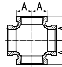
Cross
