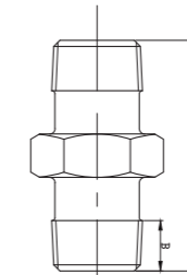
Hexagon Nipple
