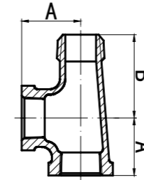
Service Tee
