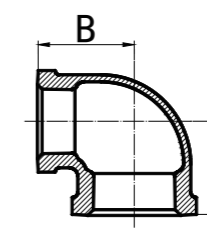
Reducing Elbow, 90°
